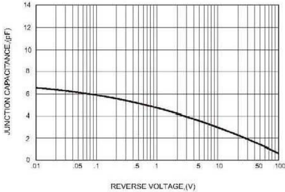
FIG.4-TYPICAL JUNCTION CAPACITANCE
